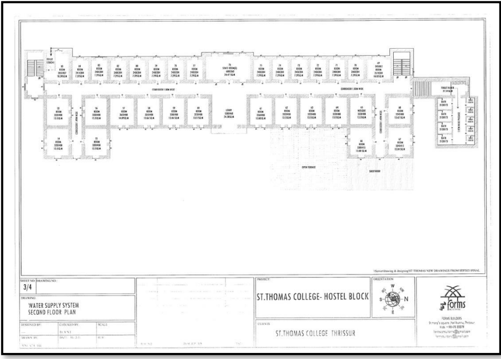
Second Floor Water Supply System in Hostel
