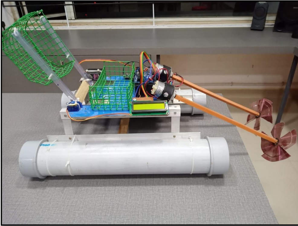
Garbage collecting from the surface of water equipment developed by St.Thomas student
