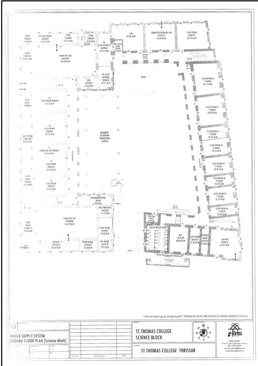
Ground Floor Water Supply System in Academic (Science ) Block
