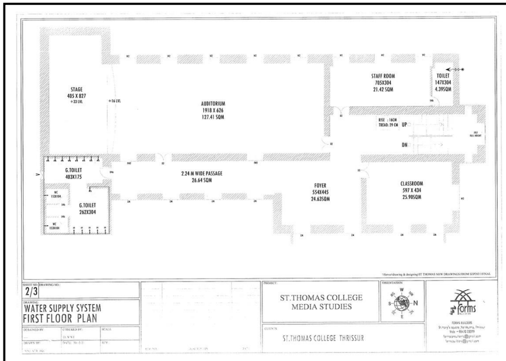
First Floor Water Supply System in Media Block
