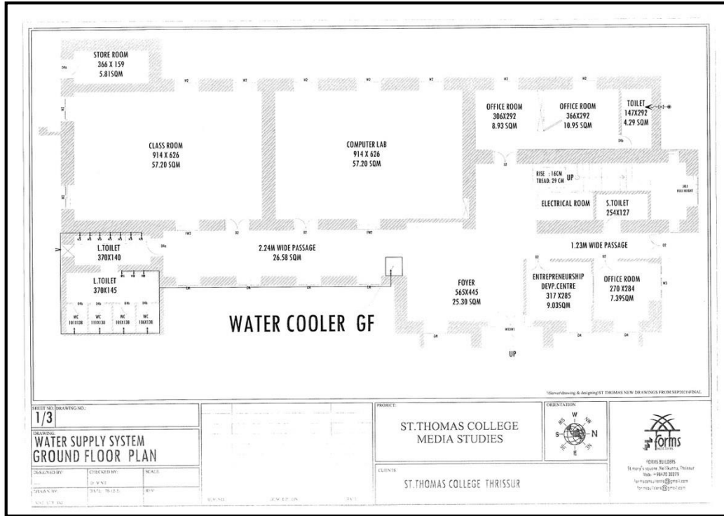
Ground Floor Water Supply System in Media Block
