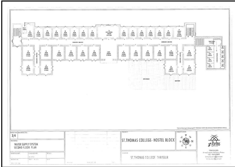
Second Floor Water Supply System in Hostel
