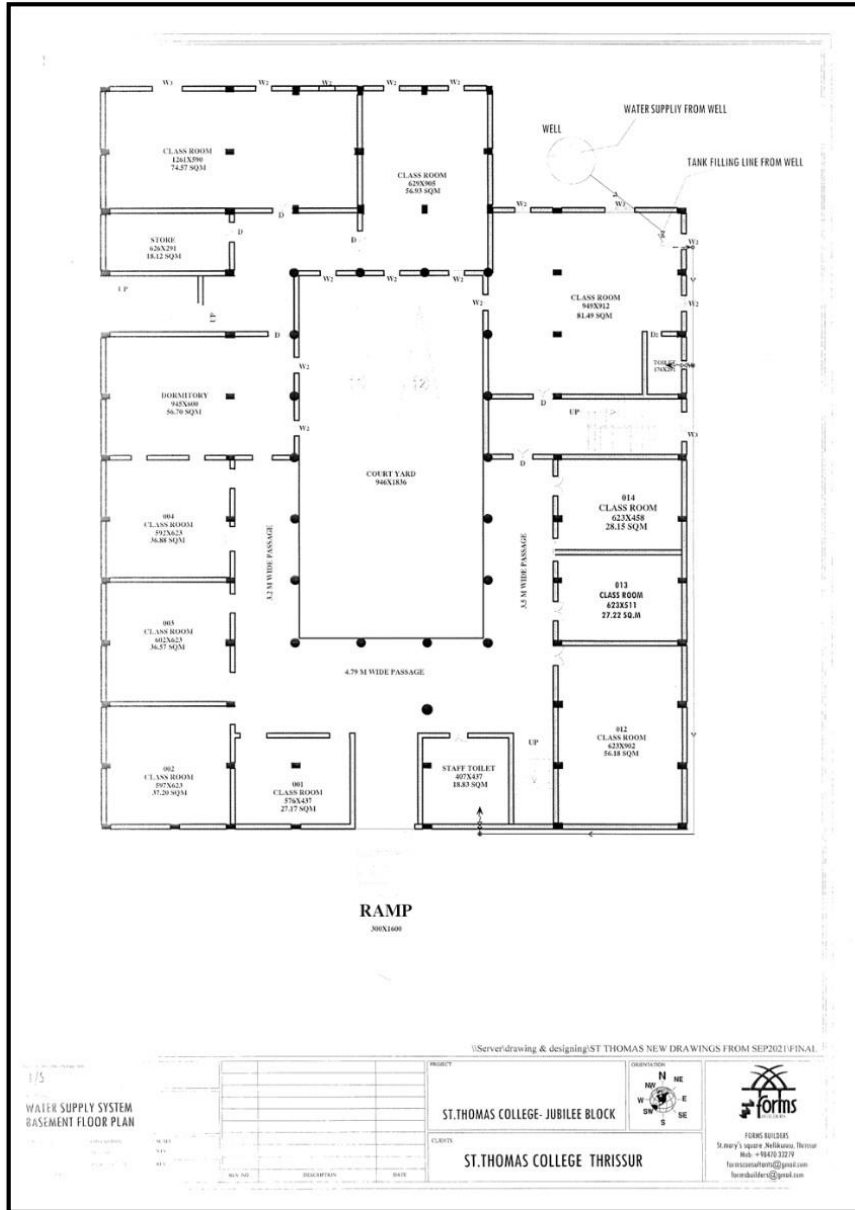
Basement Floor Water Supply System in Jubilee Block
