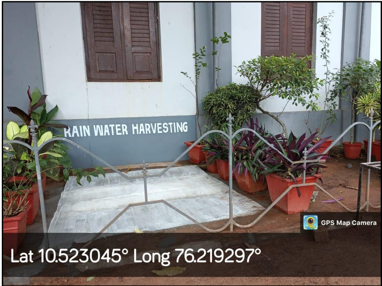
Rain Water Harvesting at Administrative Block
