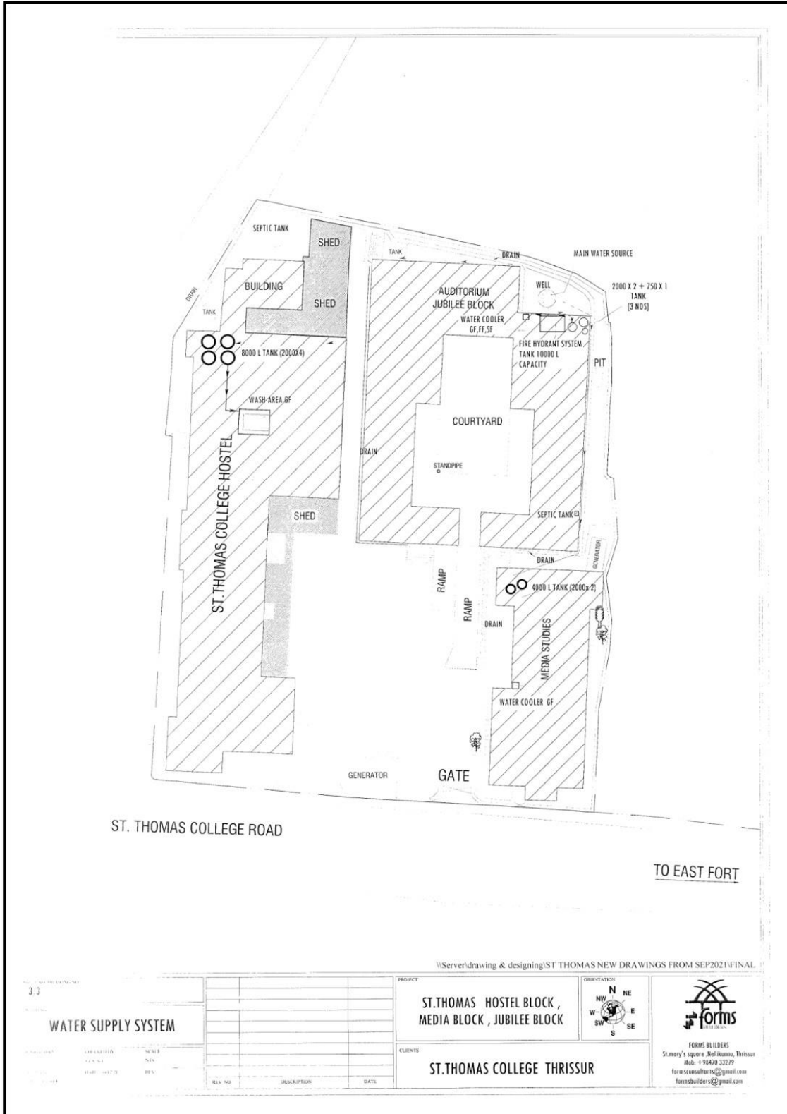
Water Supply System Hostel, Media & Jubilee Block
